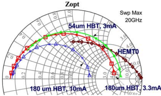
Fig. 11. Modeled optimum noise impedance Z_{\text{opt}} , 0.2–20 GHz, at 15 K for the cases shown in Table II. Note that if this impedance was expressed as an admittance, i.e., Y_{\text{opt}} , then G_{\text{opt}} is more constant with frequency than R_{\text{opt}} .
