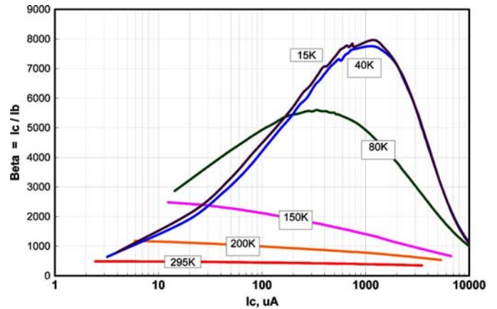
Fig. 3. \beta = I_C/I_b as a function of collector current at six temperatures for an IBM 8-HP 54- \mu\text{m} SiGe transistor. The peak cryogenic \beta at I_C = 1000 \mu\text{A} thus occurs at a current density of 0.15 \text{ mA}/\mu\text{m}^2 , which is well below the current density for peak g_m or F_t . \beta is a function of current density and, thus, for example, a 10 \times 18 \times 0.12\text{-}\mu\text{m}^2 device would have peak \beta for temperatures < 40 \text{ K} at a collector current of 3.3 mA.
